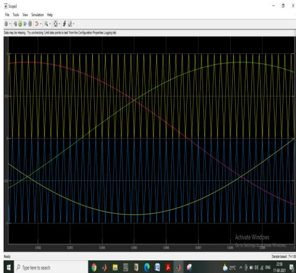
PWM waveform
