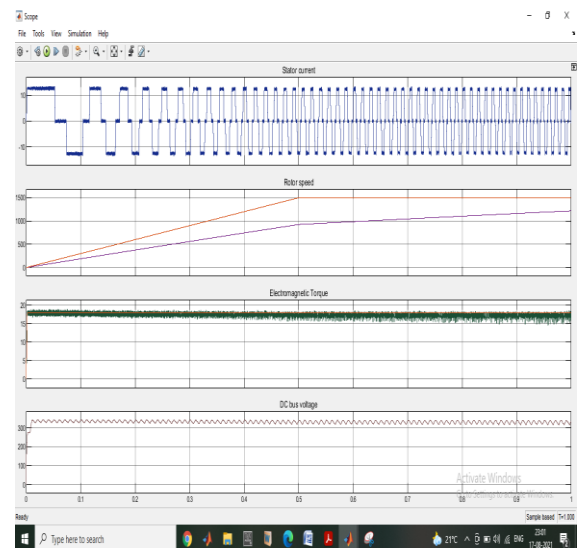
BLDC motor Current, speed torque, and voltage waveforms.
