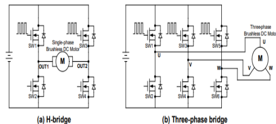
Figure 13: Driving Circuit for a BLDC motor
