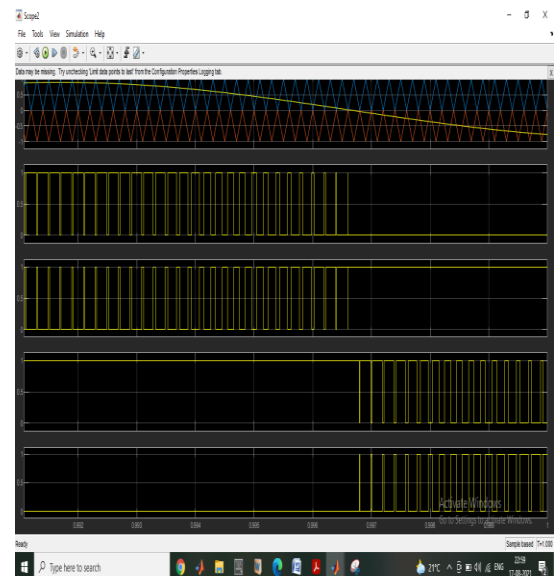
Gate pulses of three phases.
