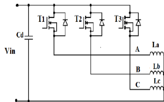
Figure 17: Half bridge-type driver circuits.
