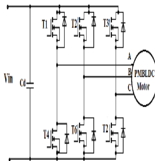
Figure 18: Full Bridge type driver circuits.
