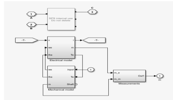
Figure 21: Electrical and Mechanical parameters of BLDC in SIMULINK
