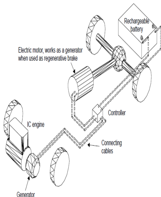
Figure 3: Series hybrid vehicle layout.
