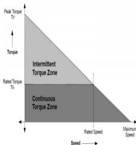
Figure 11: Torque Speed Characteristics of BLDC Motor.
