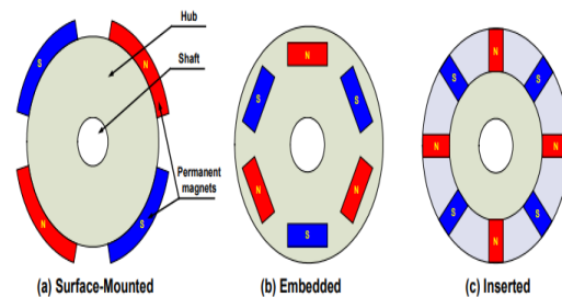
Fig. 9 Rotor Magnets in BLDC Motor.
