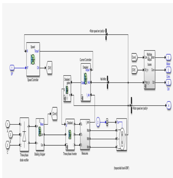
Figure 20: Complete model of BLDC Motor in SIMULINK.
