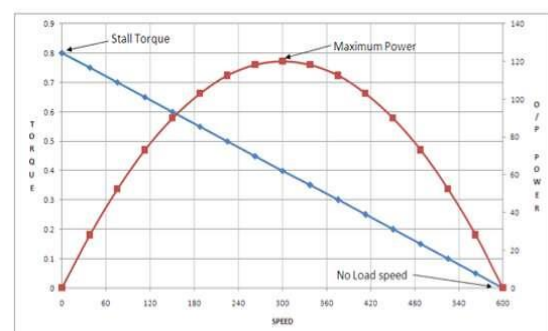
Figure 14 Speed – Torque – Power Characteristics of BLDC Motor
