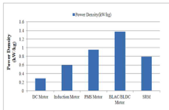
Figure. 4: Comparison of various motors for E.V. applications.
