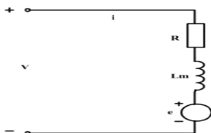
Figure 16: Equivalent circuit of BLDC motor
