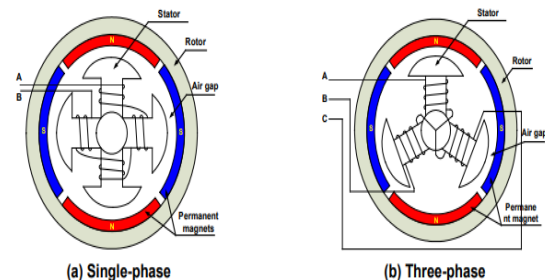
Figure 8: Single phase and Three phase Stator connections in BLDC Motor.
