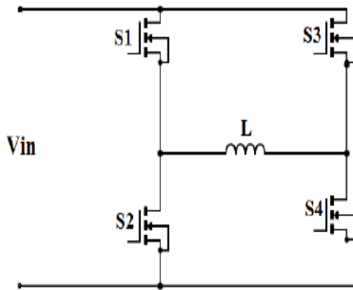
Figure 19: H-Bridge type driver circuits.
