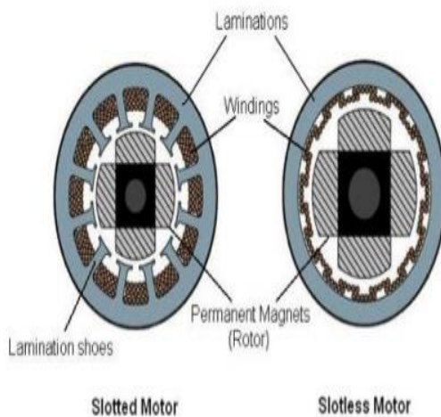
Figure 6: Two types of stators.
