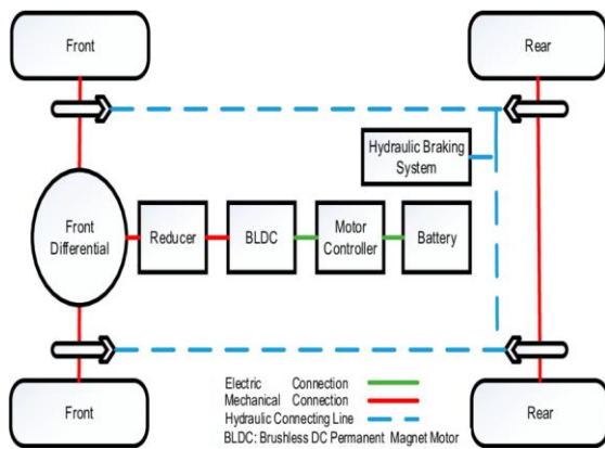
Figure 2: Electrical vehicle structure
