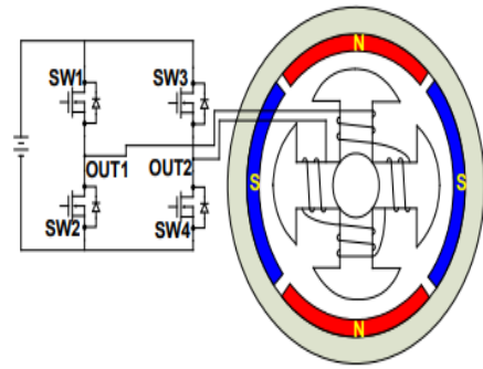
Figure 12 BLDC with Converter.
