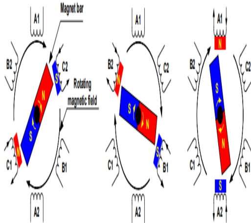
Figure 10: Rotor at various positions.
